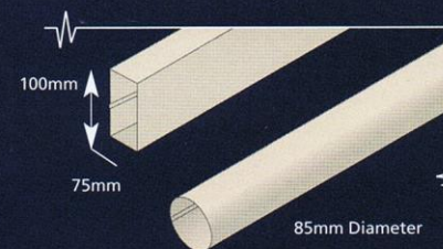
Stramit® Downpipes
